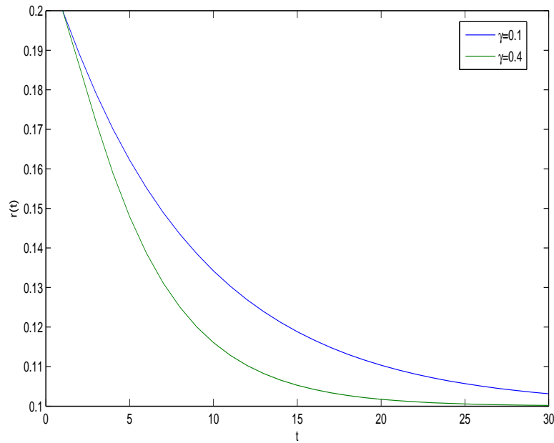
Figure 1: Different speed of convergence for different values of \gamma
